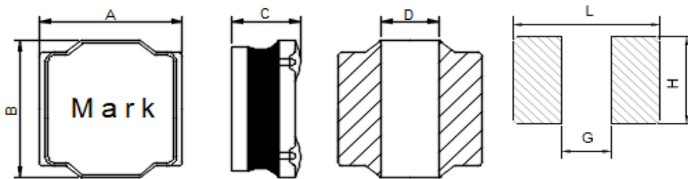
DIMENSIONS (mm)
