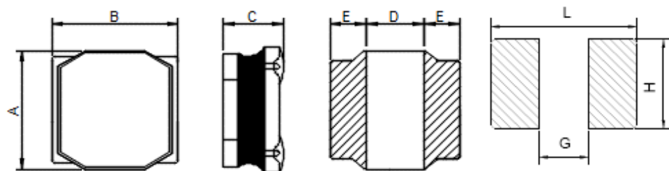
DIMENSIONS (mm)
