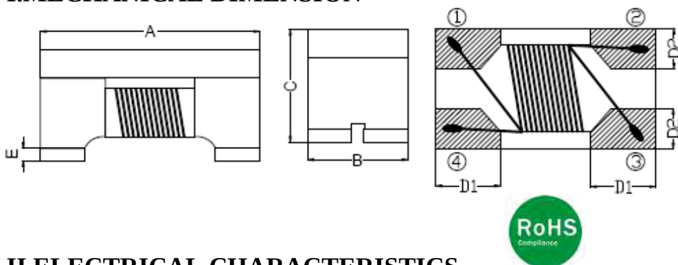
DIMENSIONS (mm)
