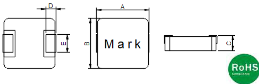
DIMENSIONS (mm)
